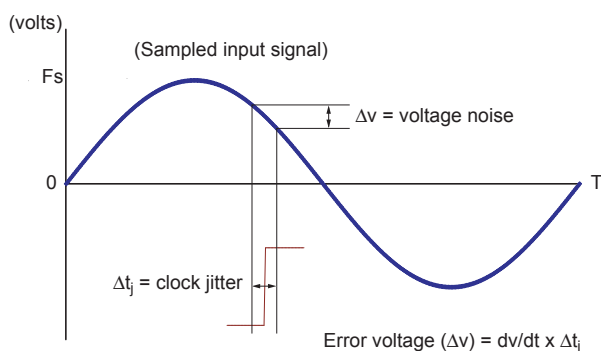
Sampling noise due to clock jitter
