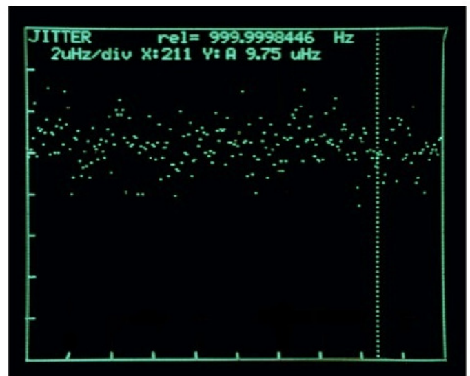
Allan variance plot
