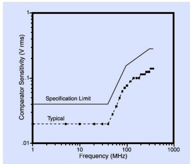
Input sensitivity
