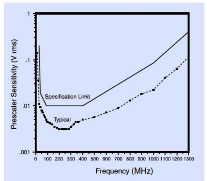
Prescaler sensitivity
